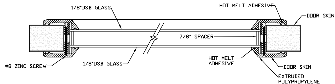
SECTION D-D 24" X 12" WINDOW DETAIL W/ 1-1/8" INSULATED GLASS N.T.S.
